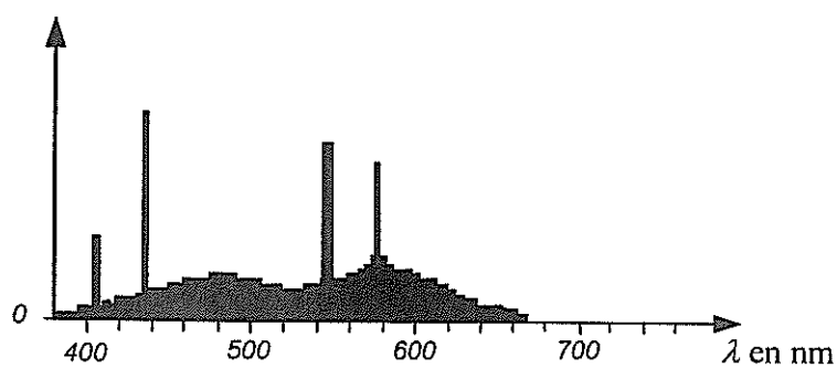
Figure 2 : tube fluorescent 2
