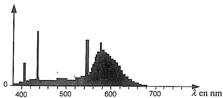
Figure 1 : tube fluorescent 1
